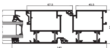
door – cross-section
