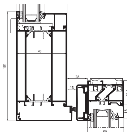
door – cross-section
